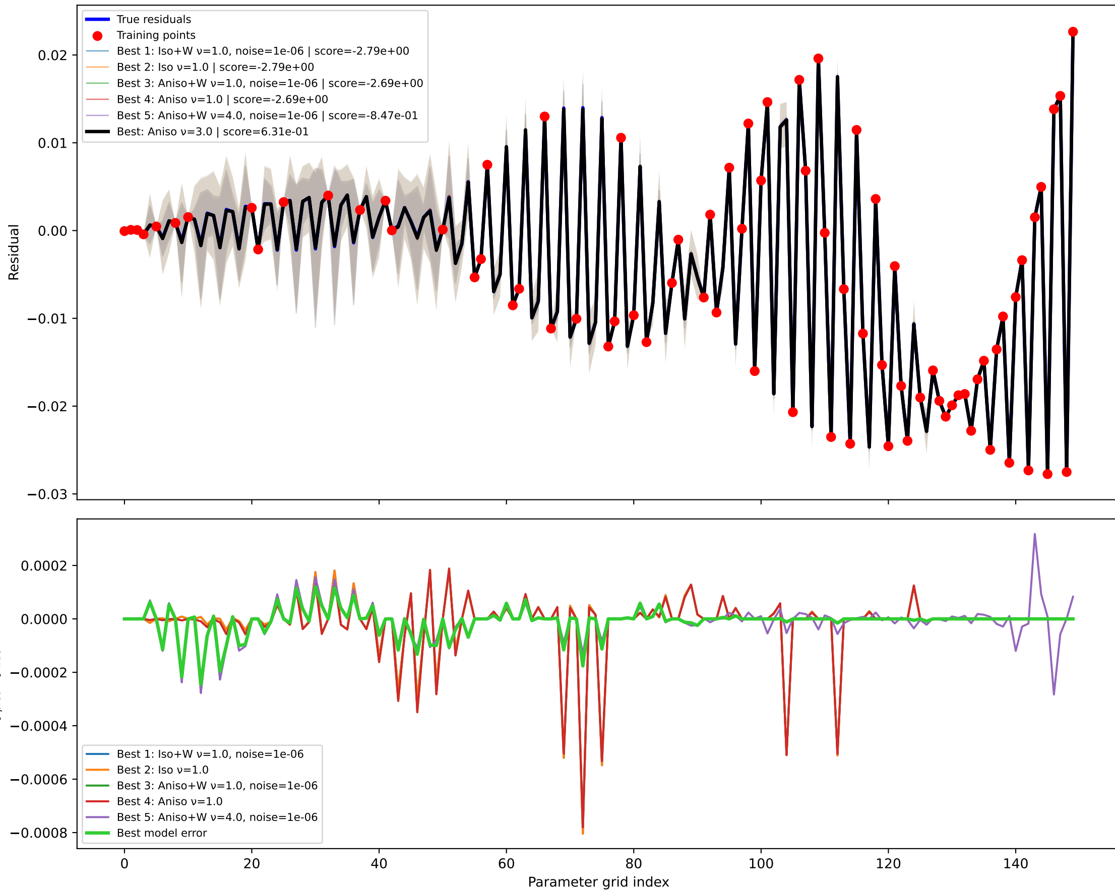
GPR kernel comparison node=16 RMSE=5.256e-05, train RMSE=6.437e-11
